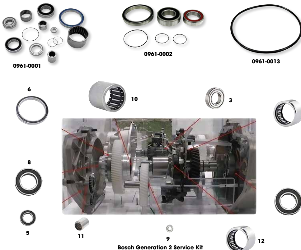
Bosch Generation 2 Service Kit
