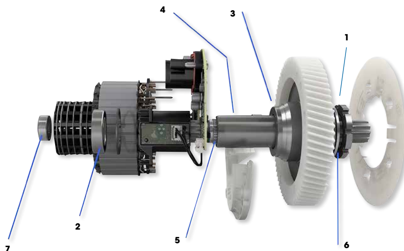
Bosch Generation 3 Service Kit
